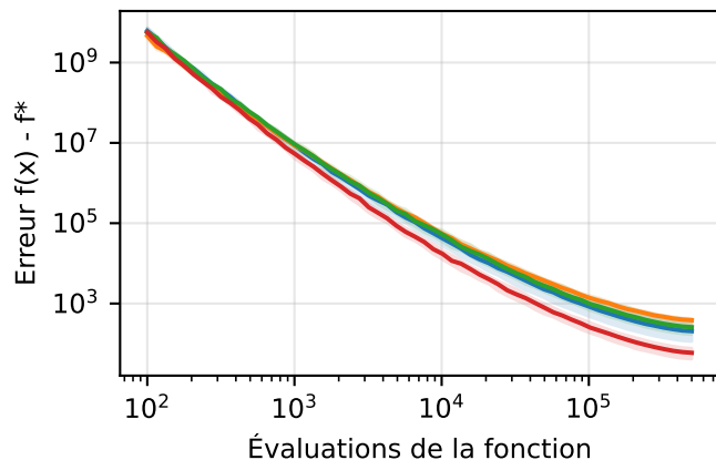
Shifted Rosenbrock
