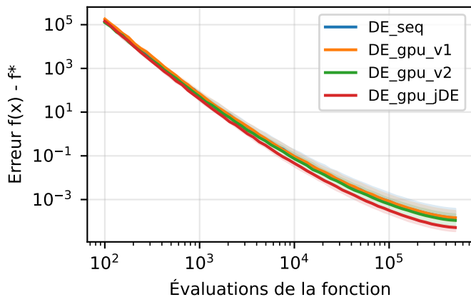
Shifted Sphere
