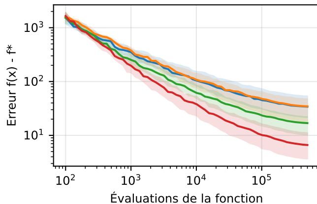
Shifted Rastrigin
