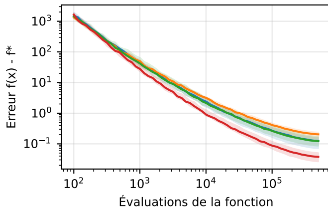
Shifted Griewank
