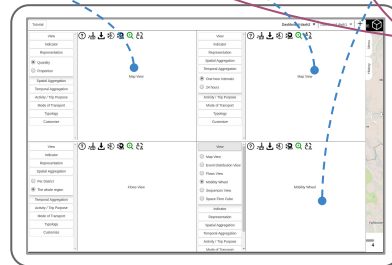
the data selector (tab-based menu)
