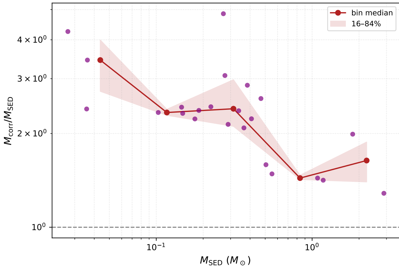
Applied correction factor — real Aquila (4D)
