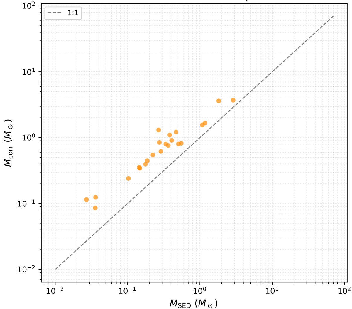
Corrected vs SED mass — real Aquila (4D)
