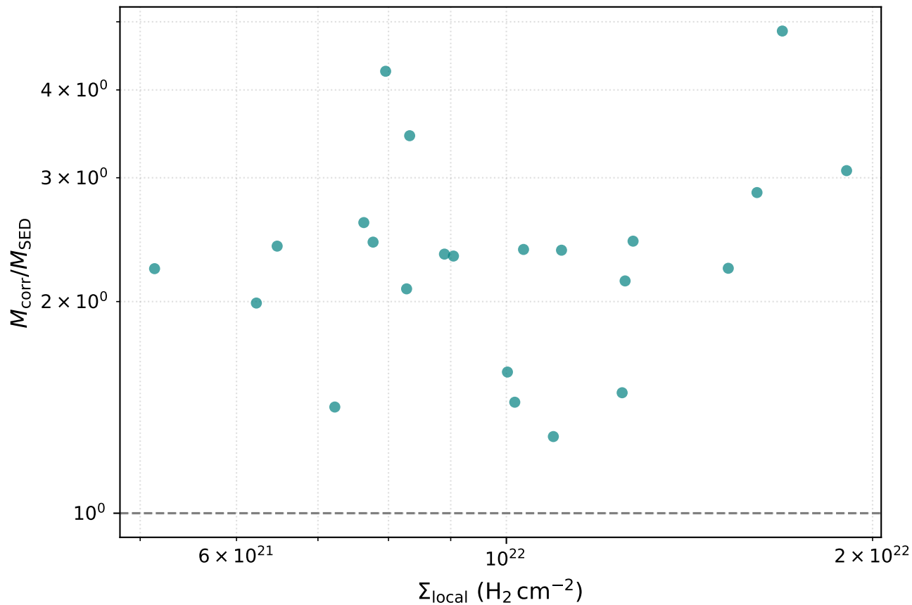
Correction vs local column — real Aquila (4D)
