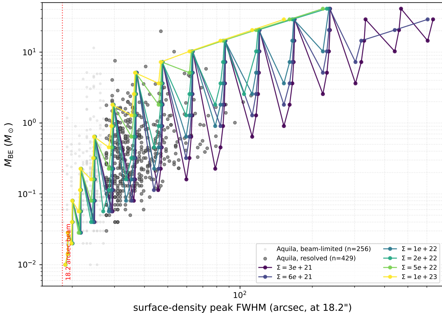
Critical-BES M(size) vs Aquila (both at 18.2 arcsec)
