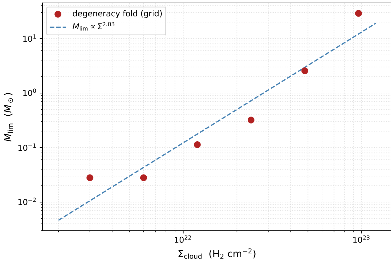
Mass-completeness limit of the correction vs cloud column
