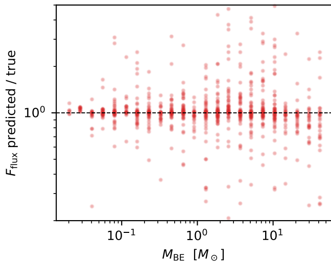
(a) F_{\text{flux}} : predicted vs. true
