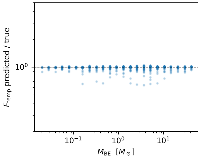
(e) F_{\text{temp}} : predicted vs. true
