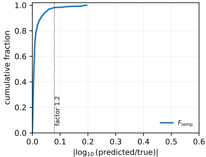
(f) F_{\text{temp}} : accuracy CDF, scatter = factor 1.06
