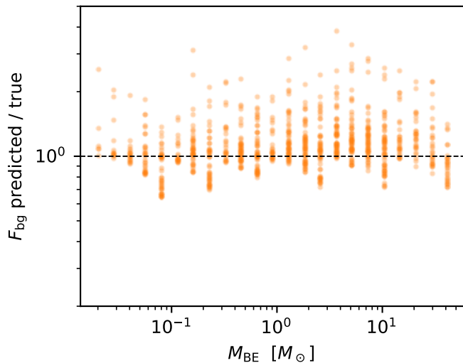
(c) F_{\text{bg}} : predicted vs. true
