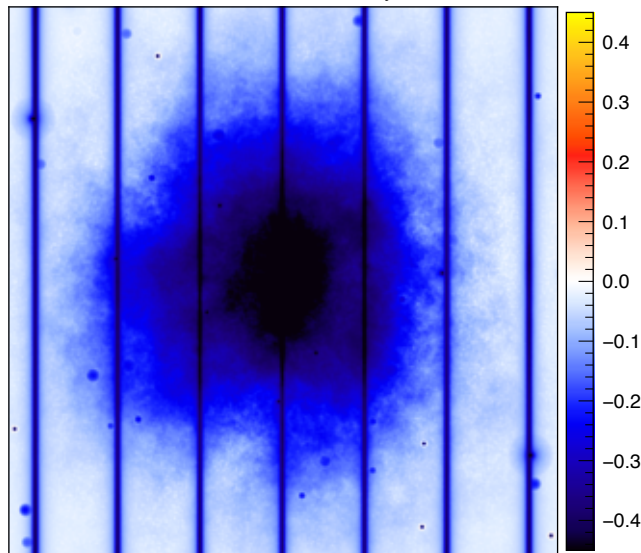
hires 13.5'' surface density
