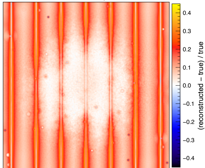
hires 13.5'' surface density, corrected
