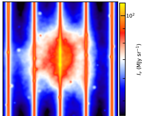
500 \mu\text{m} , 36.3 arcsec
