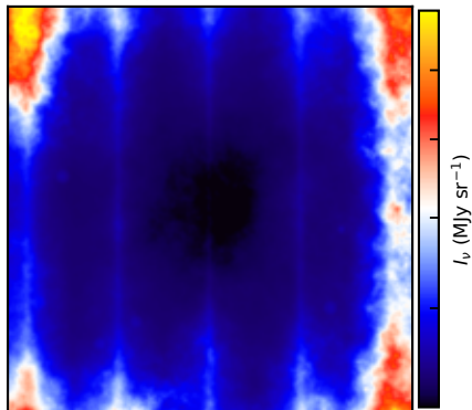
160 \mu\text{m} , 13.5 arcsec
