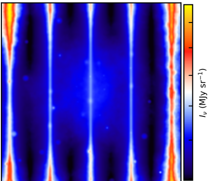
250 \mu\text{m} , 18.2 arcsec
