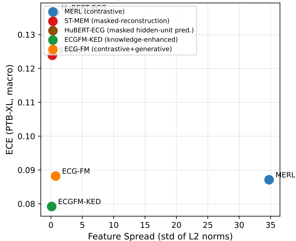
Feature Spread vs Calibration Error
