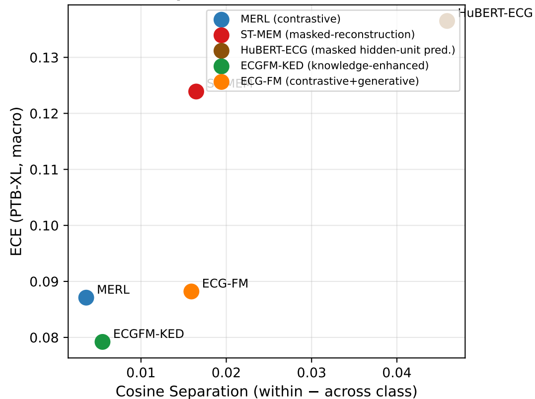
Class Separation vs Calibration Error
