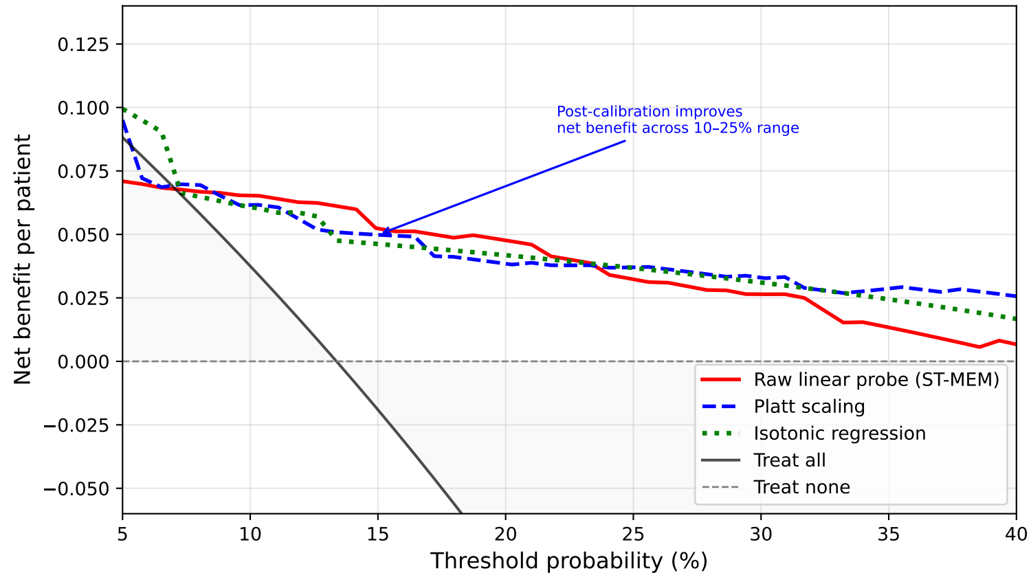
Decision-Curve Analysis: PTB-XL MI Class (ST-MEM) n_{\text{test}} = 299 , MI prevalence 13.4% ( n_{\text{pos}} = 40 ) — from real predictions
