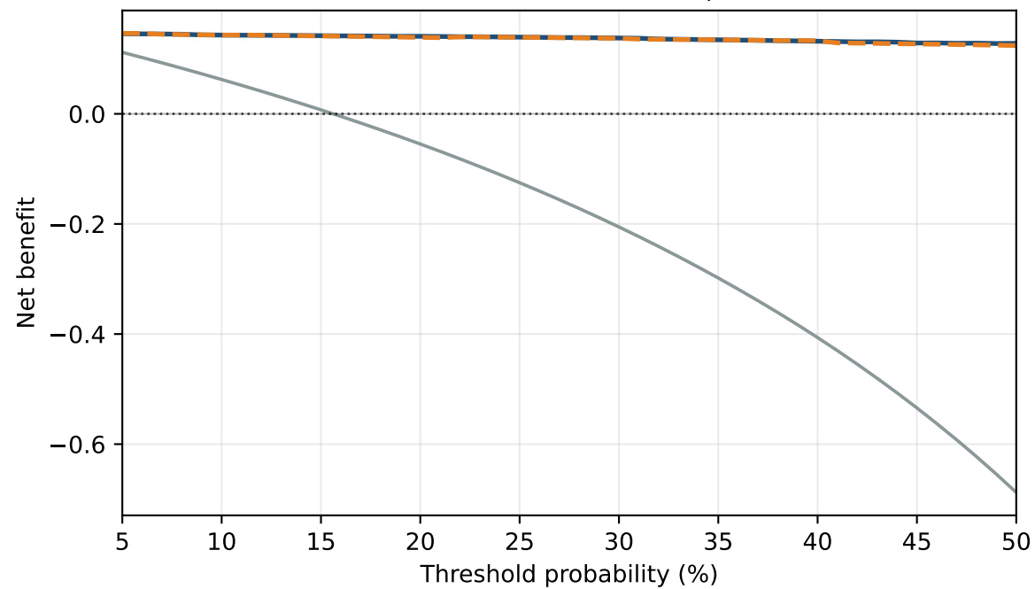
MIMIC-IV-ECG - best ECE S4D (AUROC=0.72, ECE=0.04, prev=0.13)
