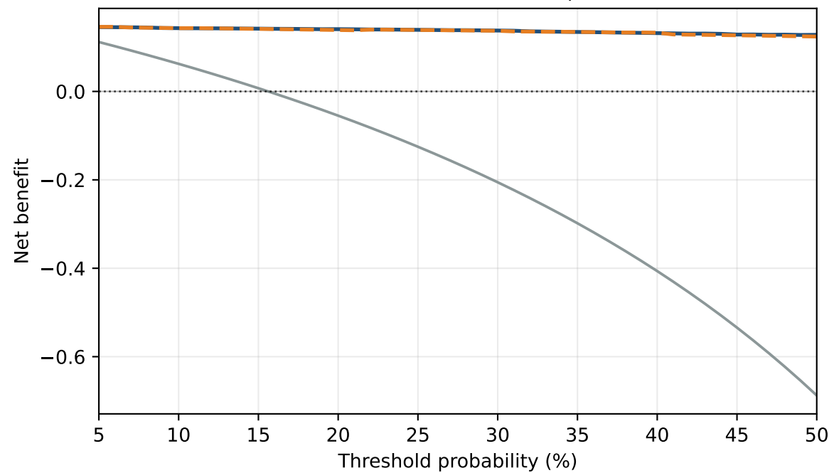
MIMIC-IV-ECG - best AUROC ST-MEM (AUROC=0.96, ECE=0.05, prev=0.13)
