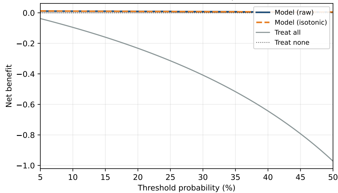
CPSC2018 - best AUROC ST-MEM (AUROC=0.98, ECE=0.02, prev=0.16)
