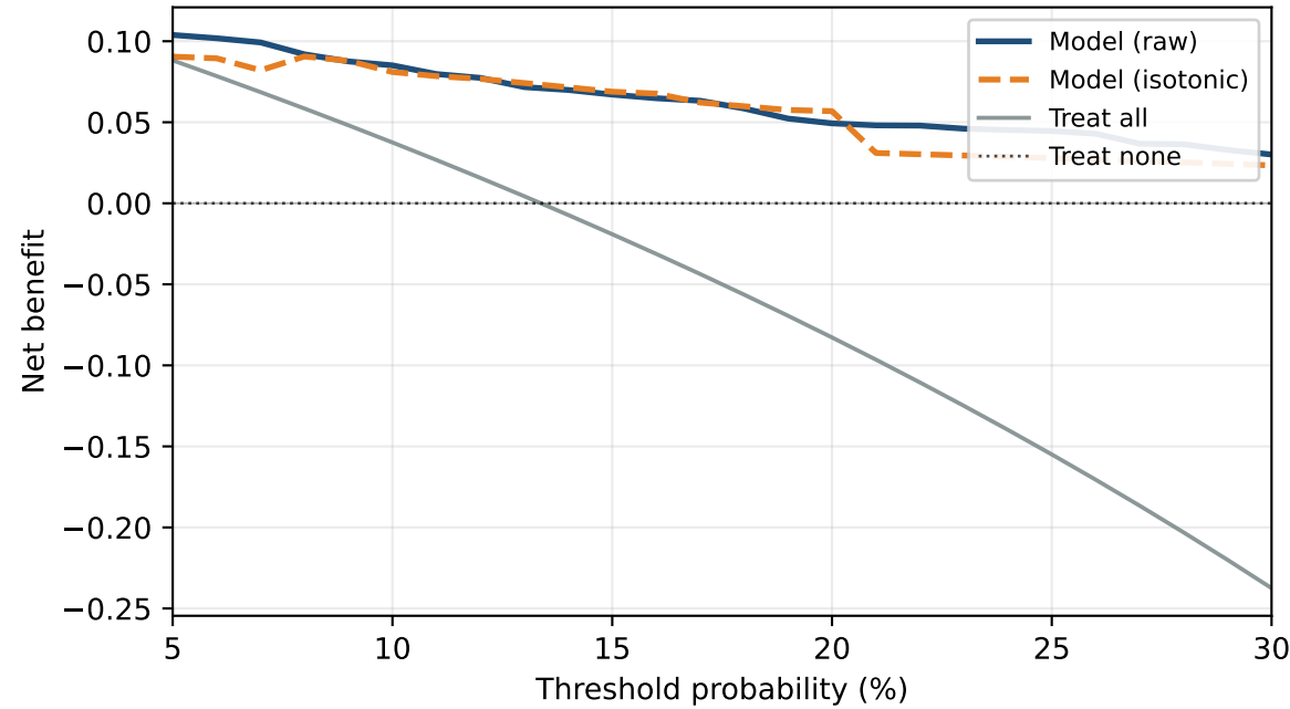
MIMIC-IV-ECG - best AUROC MERL (AUROC=0.79, ECE=0.09, prev=0.21)
