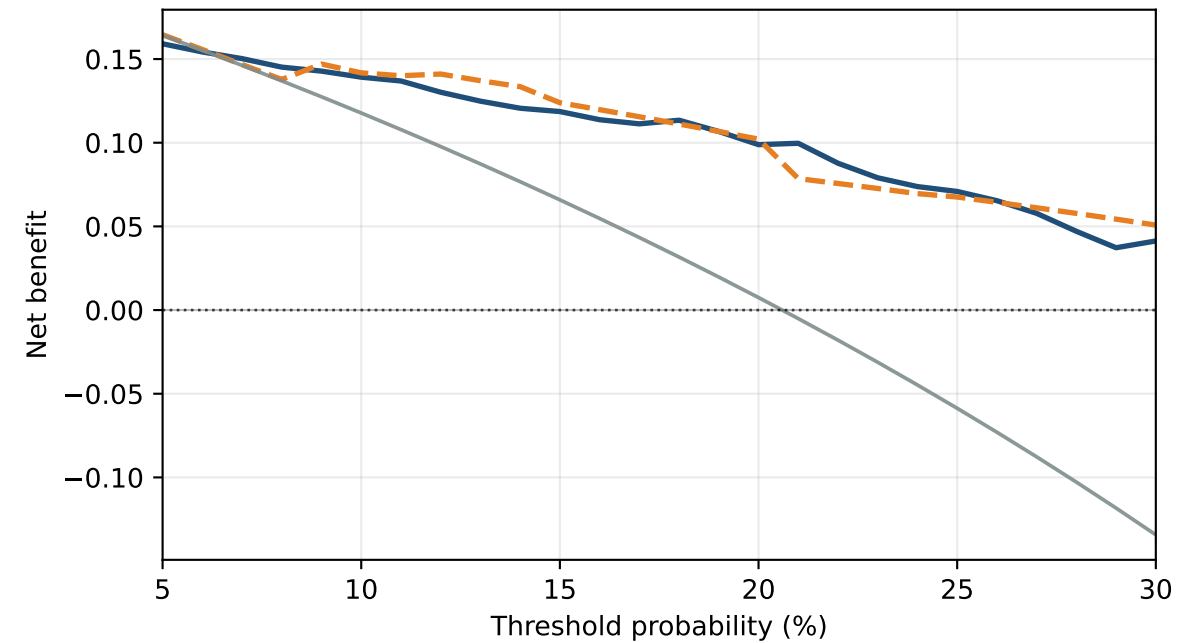
MIMIC-IV-ECG - best ECE S4D (AUROC=0.78, ECE=0.05, prev=0.21)
