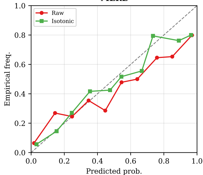
ECGFM-KED
