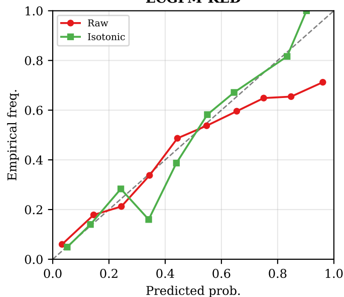
ECGFM-KED
