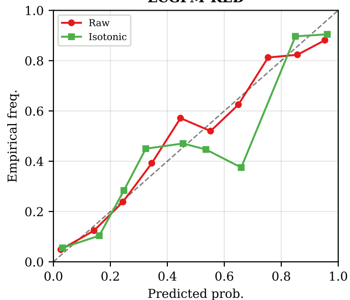
ECGFM-KED
