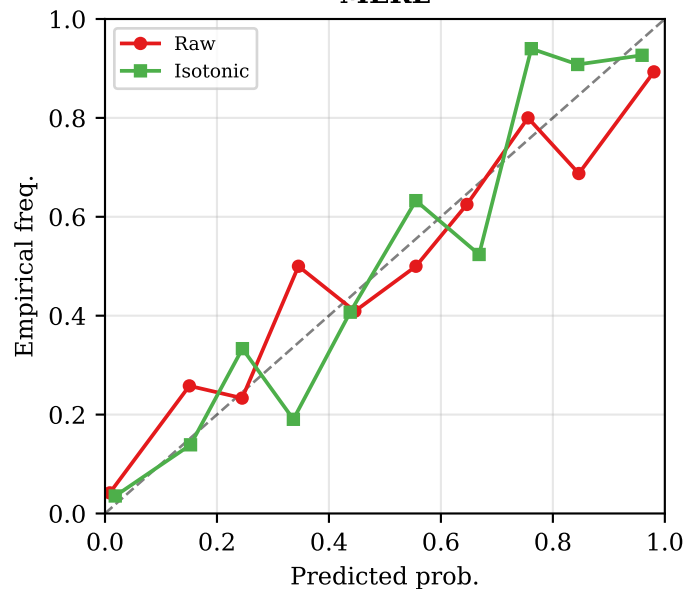
ECGFM-KED
