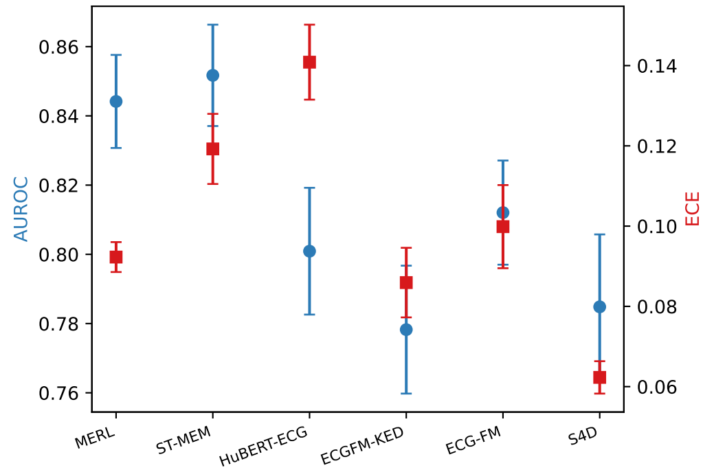
PTB-XL
