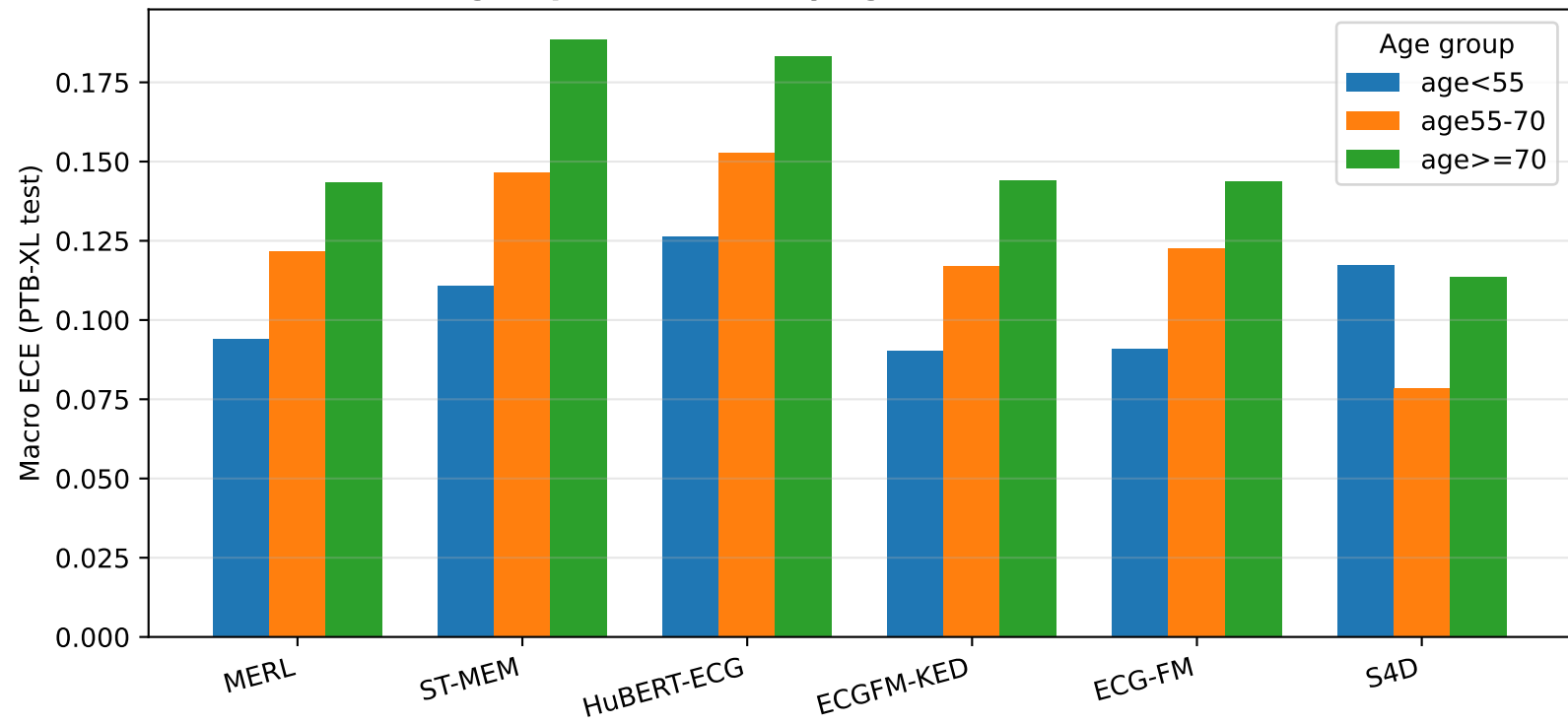
Subgroup calibration by age across all six encoders
