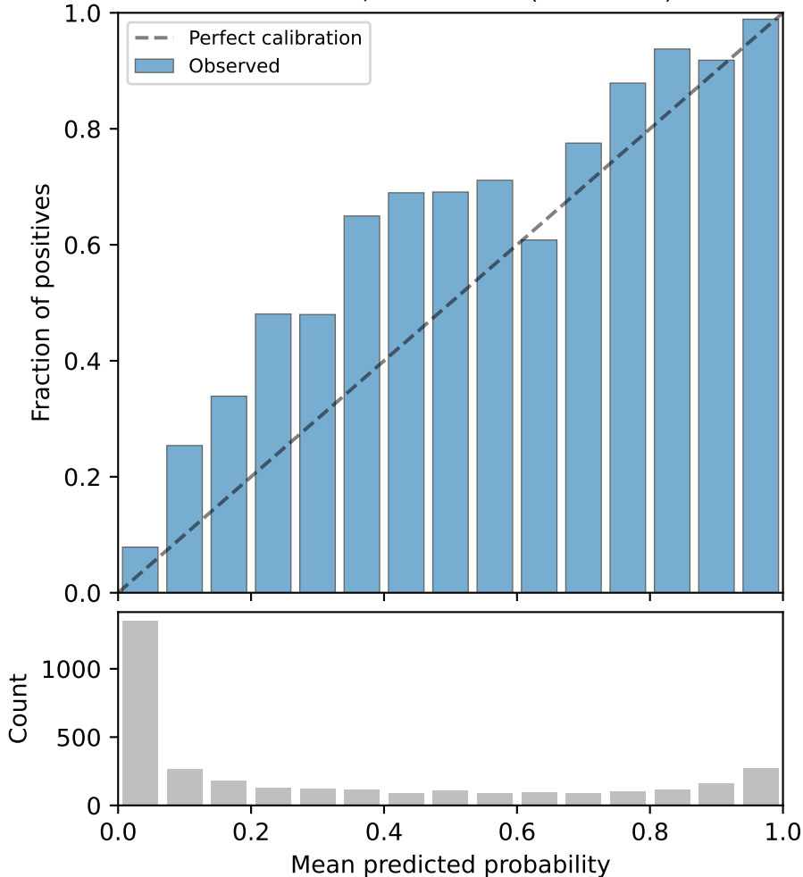
HuBERT-ECG / PTB-XL / NORM ECE=0.105, SCE=-0.104 (underconf.)
