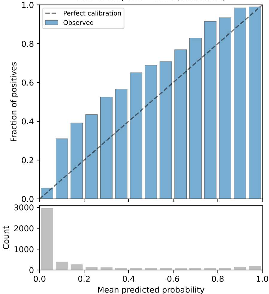
HuBERT-ECG / CODE-15% / 1dAVb ECE=0.095, SCE=-0.095 (underconf.)
