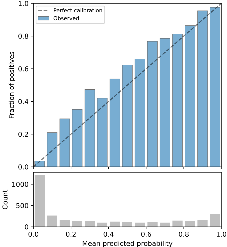
ECGFM-KED / PTB-XL / NORM ECE=0.060, SCE=-0.060 (underconf.)
