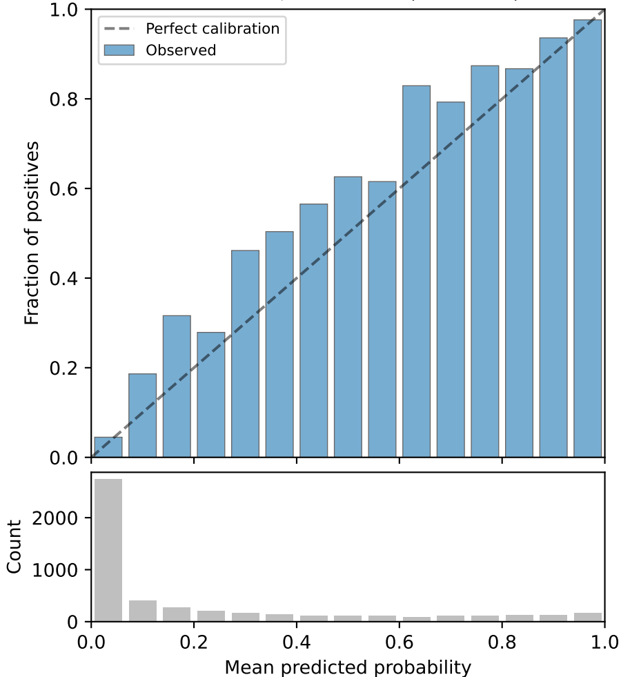
ECGFM-KED / CODE-15% / 1dAVb ECE=0.061, SCE=-0.061 (underconf.)
