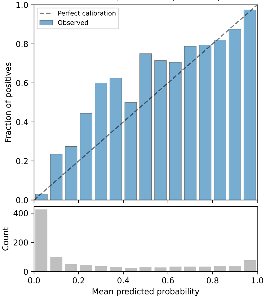
ECGFM-KED / CPSC2018 / arrhythmia_0 ECE=0.074, SCE=-0.071 (underconf.)
