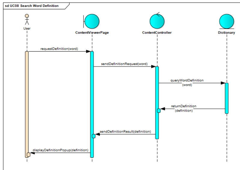
Figure 3.15: Sequence Diagram for <Search Word Definition>
