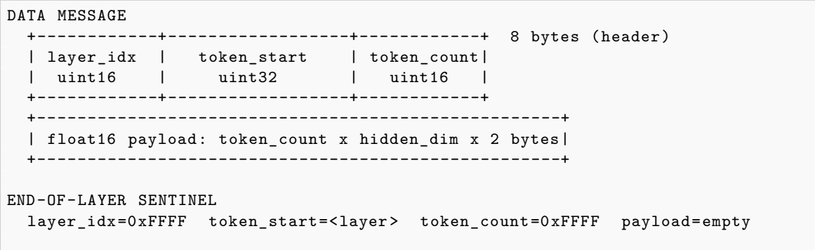
Listing 2: Wire message formats. All integers are big-endian.
