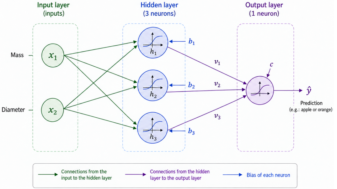
Figure 5: Pedagogical 2–3–1 architecture used to introduce neural-network computation. The two inputs — mass and diameter — feed three neurons in the hidden layer. Their activations h_1, h_2, h_3 are then combined by the output neuron to produce the prediction \hat{y} . Every connection has an adjustable weight, and every neuron has a bias.
