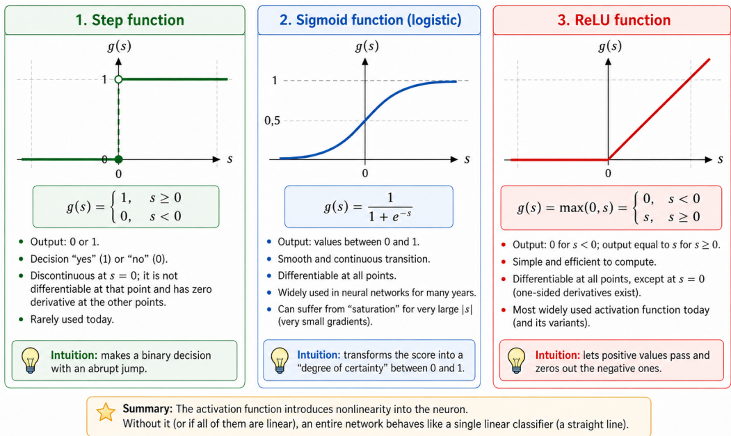
Figure 4: Comparison of three activation functions commonly used in introductory discussions of neural networks. The step function makes an abrupt decision; the sigmoid provides a smooth transition between 0 and 1; and ReLU suppresses negative inputs while preserving positive ones. Nonlinear activations prevent a stack of layers from collapsing into a single affine transformation.
