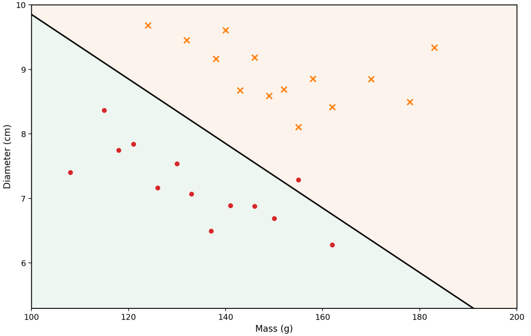
Figure 2: Example of a linear classifier in the mass–diameter plane. The straight line acts as a decision boundary: points in one half-plane receive one class, whereas points in the opposite half-plane receive the other. The decision therefore depends only on which side of the line contains the point.
