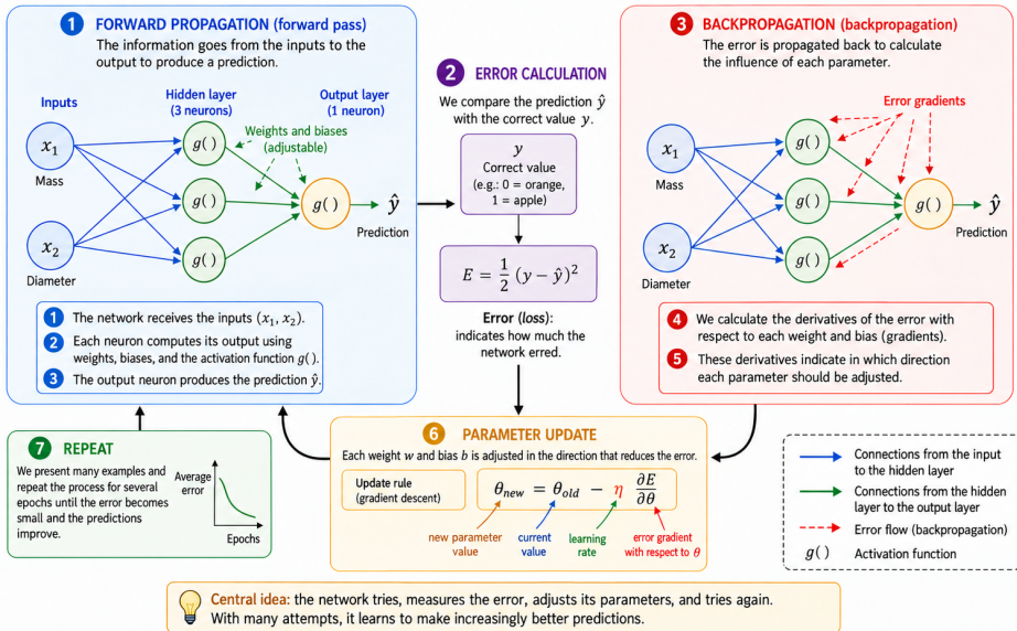
Figure 6: Basic training cycle of a neural network. The forward pass transforms the inputs into a prediction; the loss function measures the discrepancy between prediction and target; backpropagation computes gradients using the chain rule; and gradient descent uses those gradients to update weights and biases. Repeating this cycle over many epochs is what we call learning.
