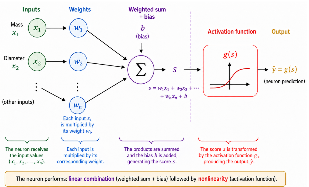
Figure 3: Schematic operation of an artificial neuron. Each input x_i is multiplied by a weight w_i ; the products are added to the bias b to produce the score s . The activation function g then transforms this score into the output \hat{y} = g(s) , which can be used as an intermediate quantity or as the final prediction.
