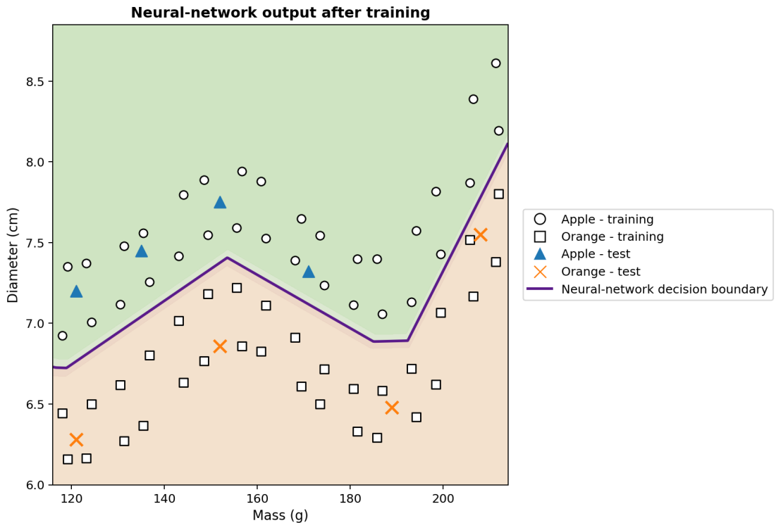
Figure 7: Python output after training the neural network. The synthetic data set contains 64 training examples spread over a broad region of the mass–diameter plane and eight additional examples reserved for an illustrative test. The highlighted curve is the level \hat{y} = 0.5 and represents the learned decision boundary; the shaded regions indicate the classes predicted by the network. Circles represent training apples, squares training oranges, triangles test apples, and crosses test oranges.
