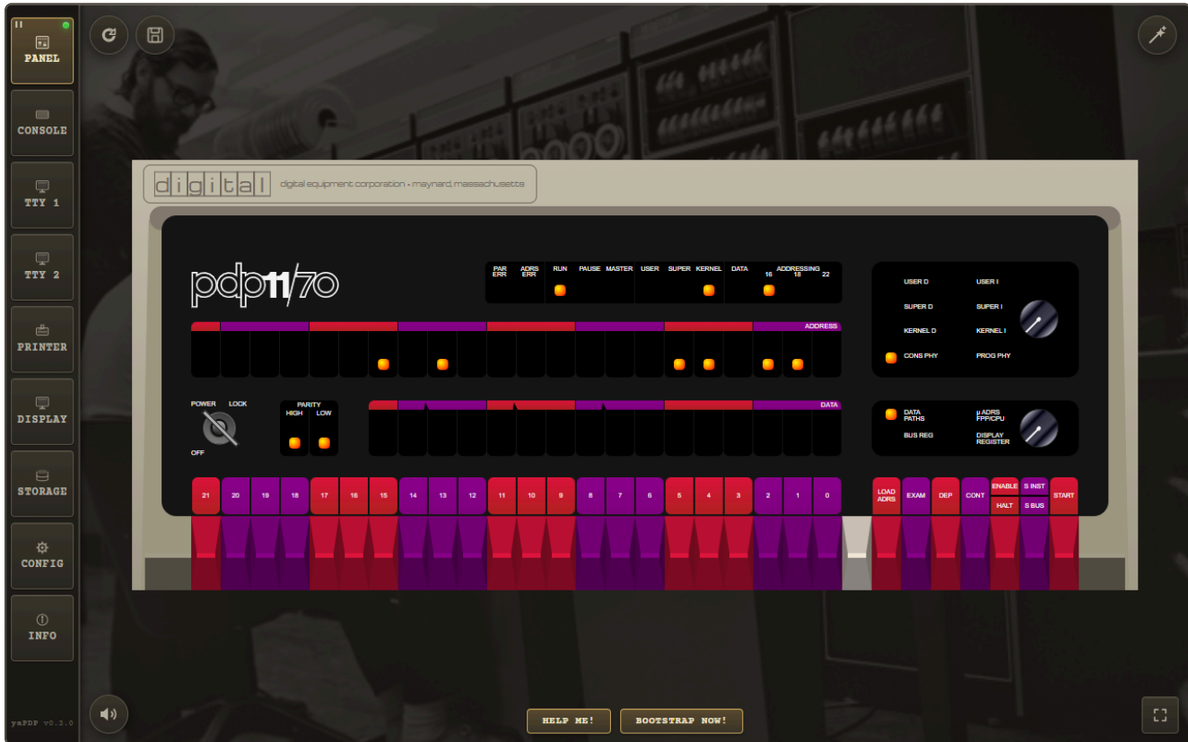
The PDP-11/70 front panel, powered on.
