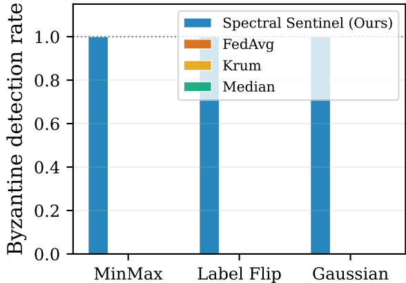
(b) Detection Rate per Attack
