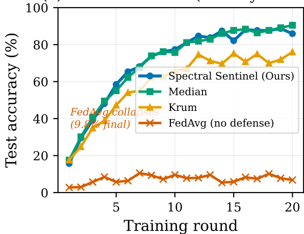
(a) Gaussian Attack (30% Byzantine)
