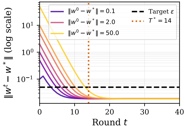
(a) Recovery from Arbitrary w^0
