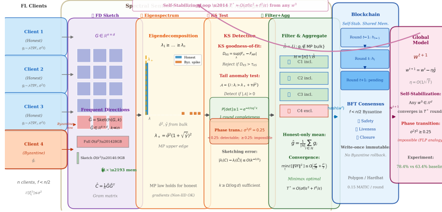
Fig. 4. Full system architecture pipeline: (1) Frequent Directions sketching compresses client gradients; (2) eigendecomposition of the Gram matrix; (3) KS test against the MP distribution; (4) Byzantine-filtered aggregation; (5) BFT on-chain checkpoint. The blockchain's write-once immutability provides the self-stabilizing shared memory substrate (Section 7).
