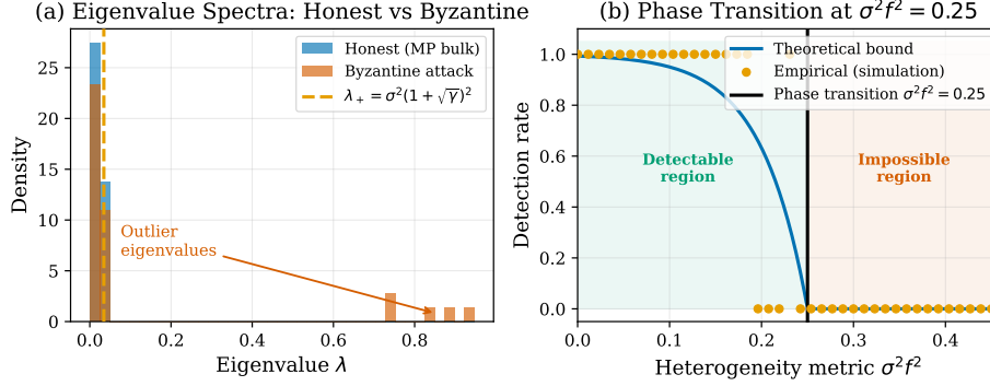
Fig. 5. Spectral detection mechanism. (a) Eigenvalue histograms for honest-only gradients (blue, MP bulk) vs. a Byzantine attack (red, outlier spikes above \lambda_+ , dashed orange). (b) Empirical detection rate vs. \sigma^2 \beta^2 : below 0.25 (green region) detection exceeds 96%; beyond it (red region) detection degrades to chance—the BBP impossibility (Theorem 6).
