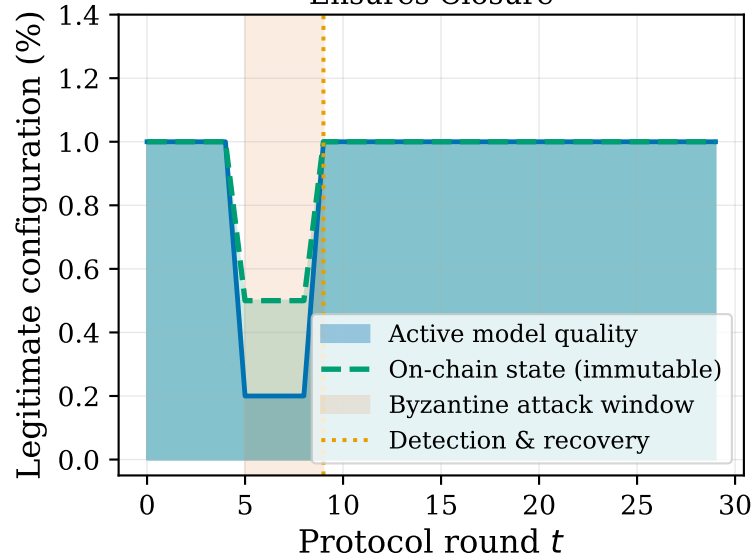
(a) Blockchain Immutability Ensures Closure
