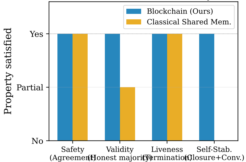
(b) Formal Properties: Blockchain vs Shared Memory
