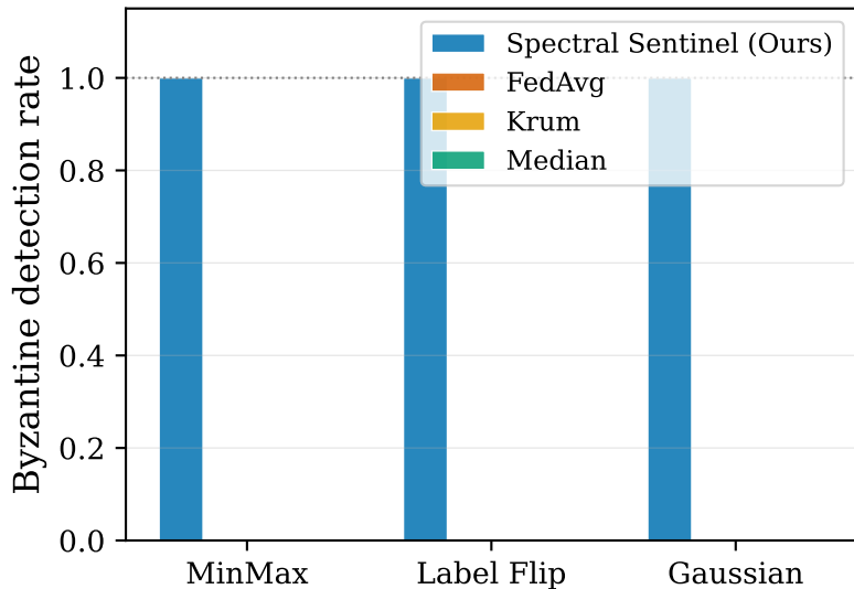
(b) Detection Rate per Attack
