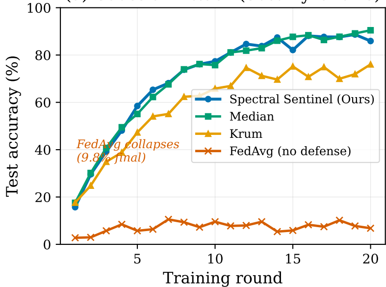
(a) Gaussian Attack (30% Byzantine)
