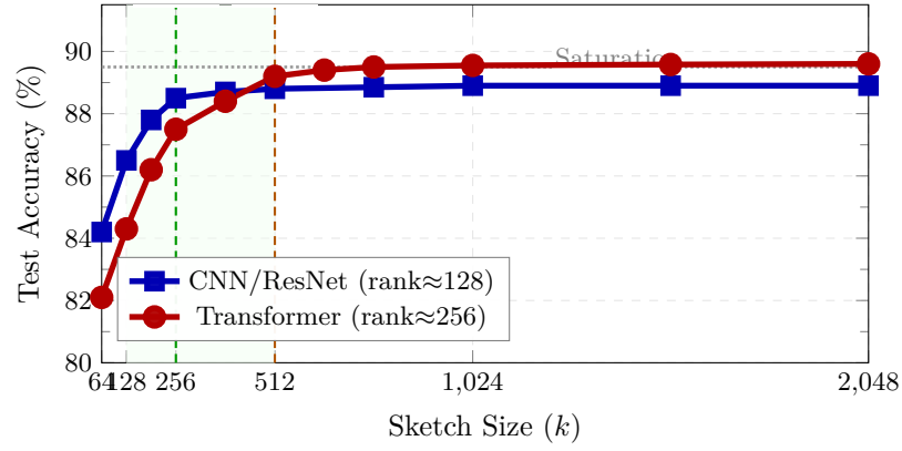
Fig. 7. Accuracy vs sketch size: CNNs saturate at k=256 (88.9%), while transformers require k=512 (89.2%) for optimal performance. The 0.7% improvement from k=256 to k=512 costs 4\times memory.
