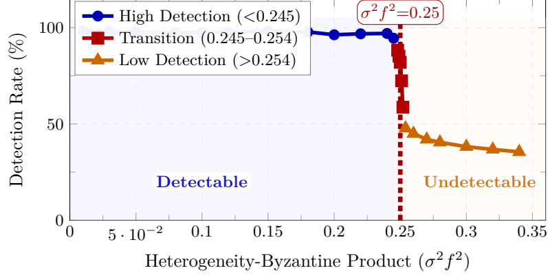
Fig. 5. Phase transition in Byzantine detection: Detection rate drops sharply from 97% to 45% at the critical threshold \sigma^2 f^2 = 0.25 , demonstrating a fundamental information-theoretic boundary.
