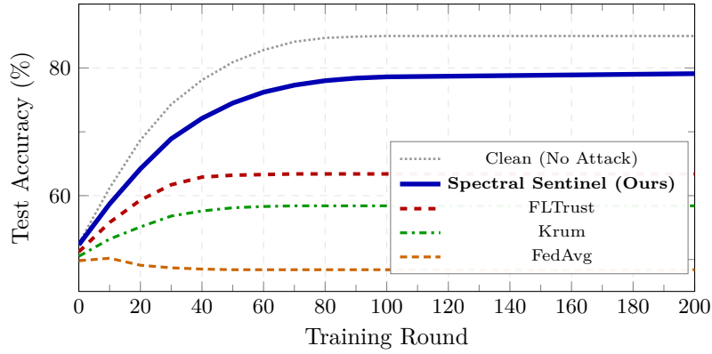
Fig. 4. Convergence under Byzantine attacks (40% adversarial clients): Spectral Sentinel achieves 79.1% accuracy vs 63.4% for best baseline (FLTrust), approaching clean performance of 85.0%.
