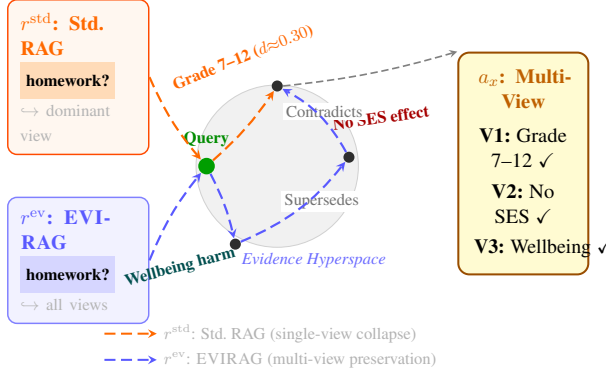
Figure 1: Evidence Hyperspace claim-graph structure. r^{\text{std}} (orange): Standard RAG takes a dominant-view path, retrieving only the most-supported claim community and collapsing the remaining views. r^{\text{ev}} (blue): EVIRAG traverses all claim communities—following contradiction and supersession edges—and preserves each conflicting viewpoint through to the multi-view answer a_x .
