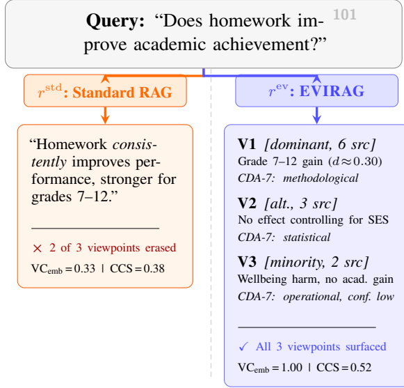
Figure 1: Epistemic collapse vs. disagreement-aware generation on a contested query. r^{\text{std}} (Standard RAG): returns one fluent answer, erasing minority viewpoints and suppressing scientific disagreement. r^{\text{ev}} (EVIRAG): surfaces three distinct viewpoints with source counts, CDA-7 causal attribution, and evidence-structured confidence. \text{VC}_{\text{emb}} and CCS values are on the homework-effectiveness query.
