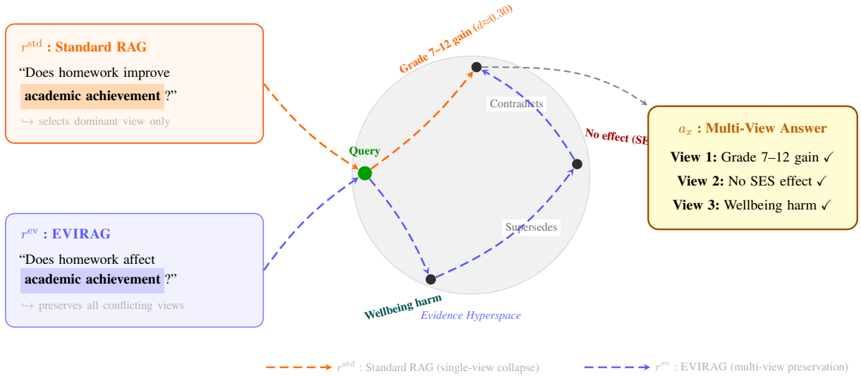
Figure 1: The claim graph structure of the Evidence Hyperspace. r^{\text{std}} : Standard RAG takes a dominant-view path, selecting only the most-supported claim community and collapsing all other views. r^{\text{ev}} : EVIRAG traverses all claim communities—following contradiction and supersession edges—and preserves each conflicting viewpoint through to the final multi-view output.
