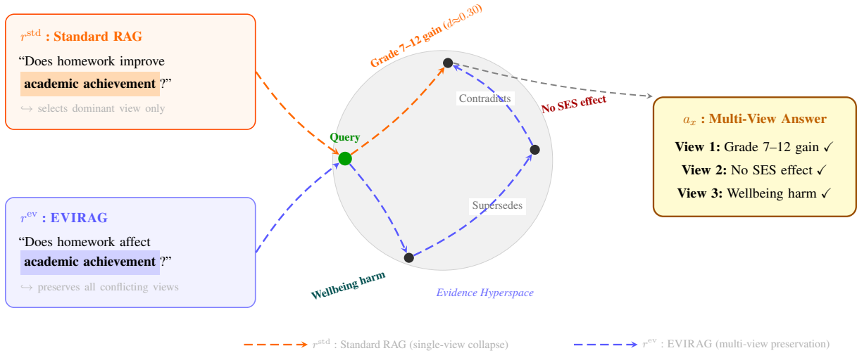
Figure 1: The claim graph structure of the Evidence Hyperspace. r^{\text{std}} : Standard RAG takes a dominant-view path, selecting only the most-supported claim community and collapsing all other views. r^{\text{ev}} : EVIRAG traverses all claim communities—following contradiction and supersession edges—and preserves each conflicting viewpoint through to the final multi-view output.
