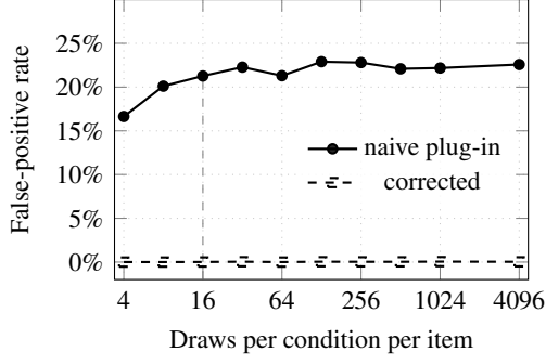
Figure 5: False-positive rate of the compatibility certificate versus sampling budget, under a null resampled from the real full-panel disclosure rates and answer-law skew (8,000 replications per point, full grid in Table 3). The dashed vertical marks the 16-draw budget used throughout. The naive certificate does not approach zero with more data: it plateaus at 21–23% out to 4,096 draws, 256 \times our budget, because near-total disclosure leaves no slack to absorb sampling noise. The per-item corrected certificate (plotted) stays at or below 0.05% (95% upper bounds at most 0.13%). The family-wise regime, used for the certified violations of Section 6, rejected none of the 8,000 replications at any draw count (Table 3).
