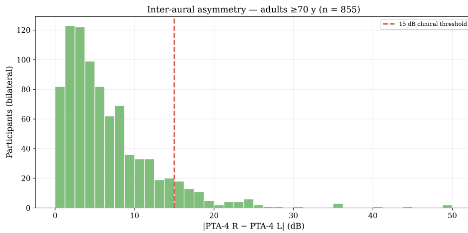
Figure 5: Inter-aural asymmetry distribution
