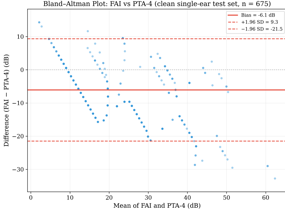
Figure 9: Bland-Altman plot: FAI vs. PTA-4 reference (adult test set)
