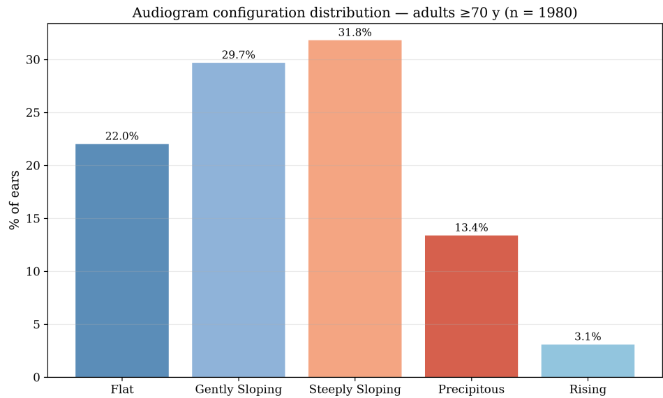
Figure 12: Configuration distribution in the adult cohort (slope = 4 kHz – 500 Hz)
