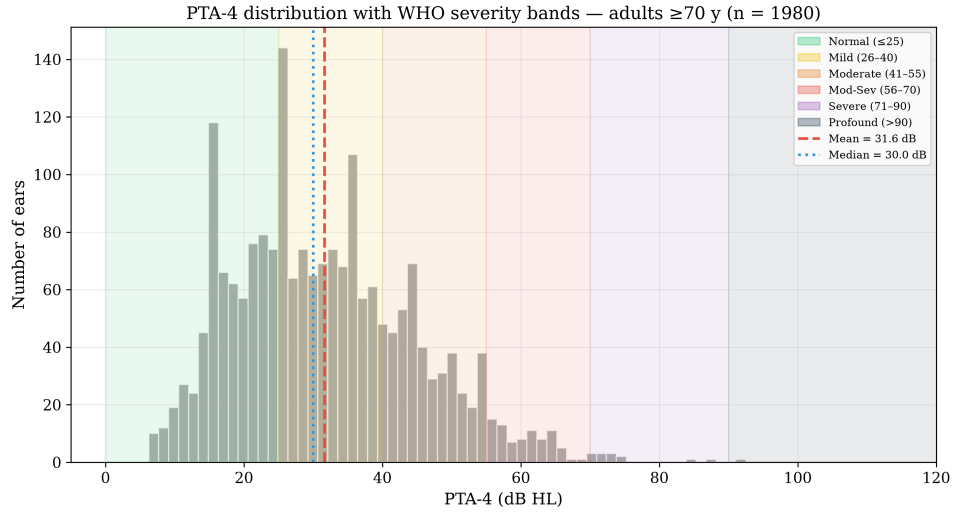
Figure 2: PTA-4 distribution with WHO severity bands
