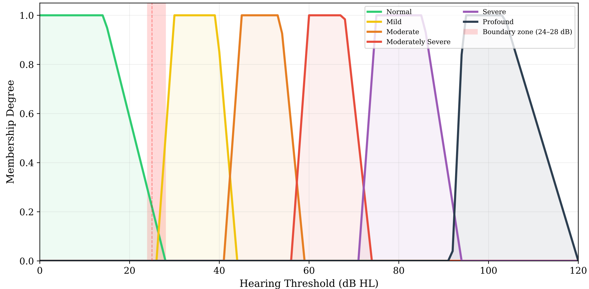
Fuzzy Membership Functions for Hearing Loss Severity (NHANES-optimized trapezoidal MFs with 2 dB overlap)
