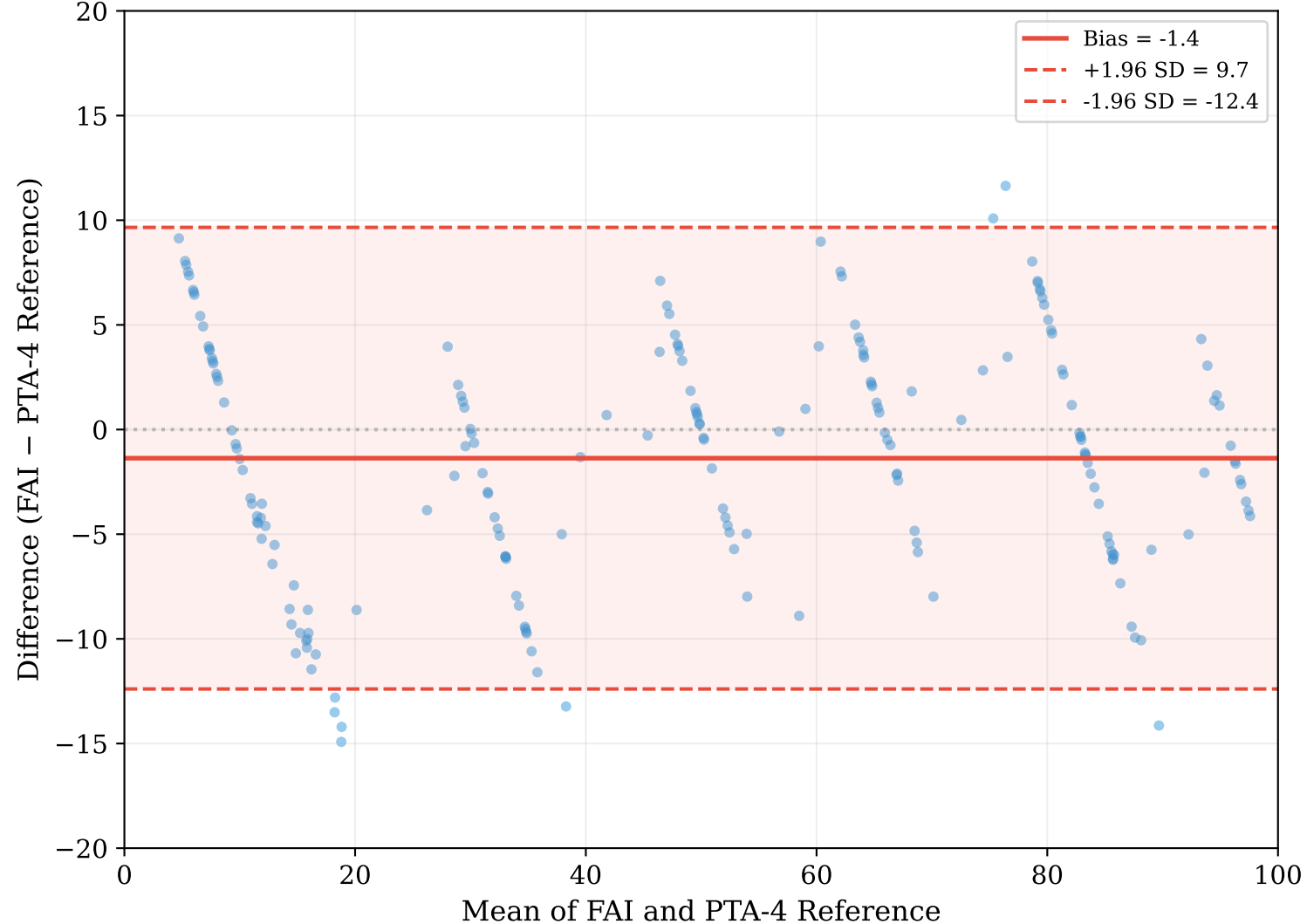
Bland-Altman Plot: FAI vs. PTA-4 WHO Reference
