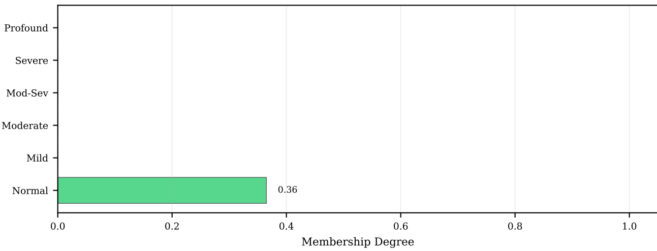
Fuzzy Classification
