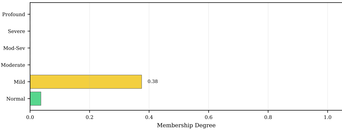
Fuzzy Classification
