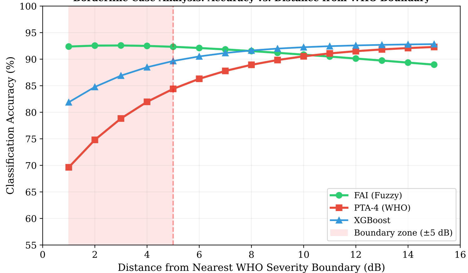
Borderline Case Analysis: Accuracy vs. Distance from WHO Boundary
