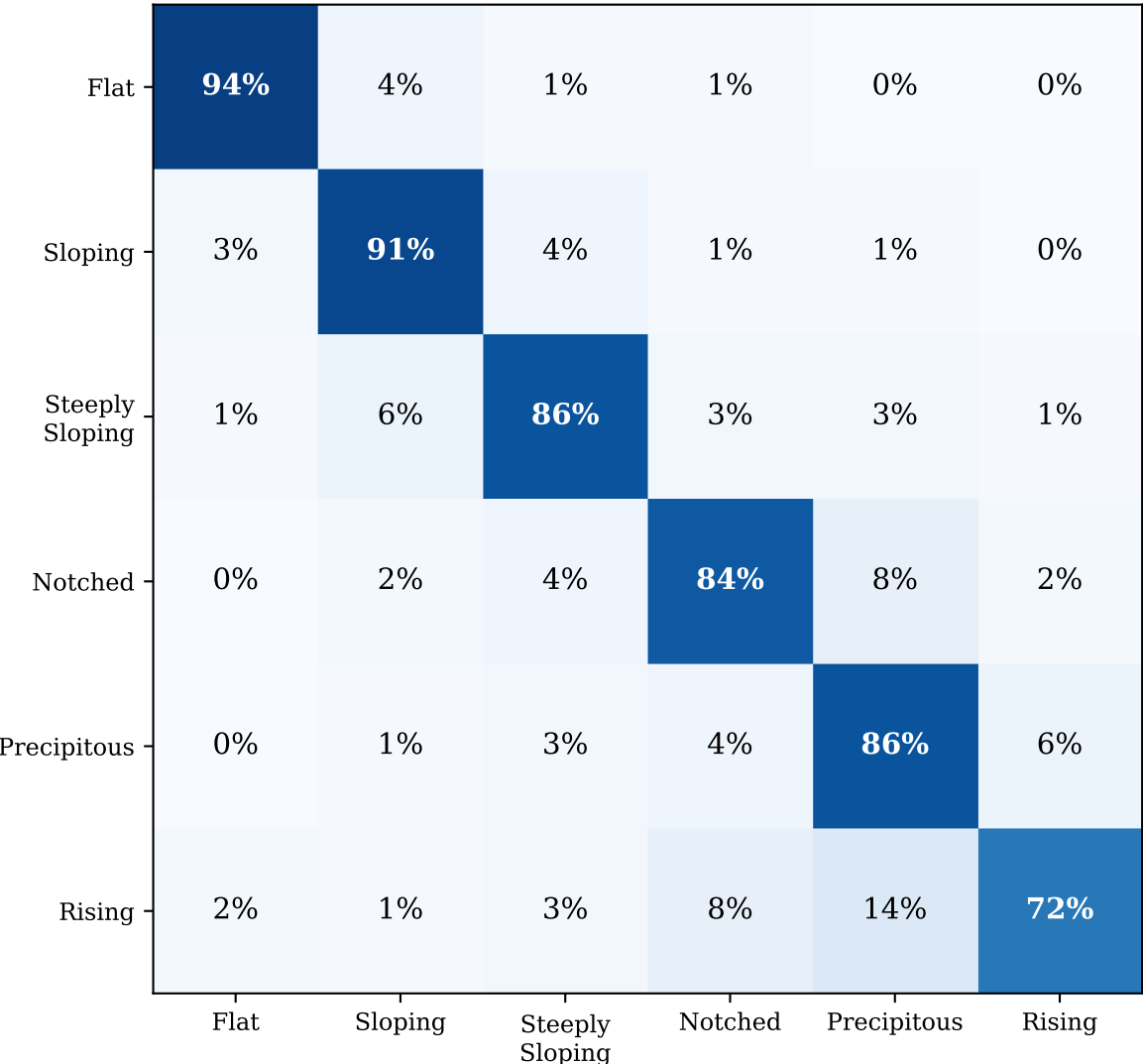
Configuration Classification Confusion Matrix (Overall Accuracy: 89.4%, \kappa = 0.86 )
