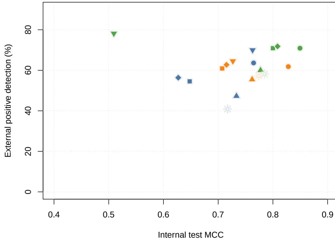
No-proxy training
