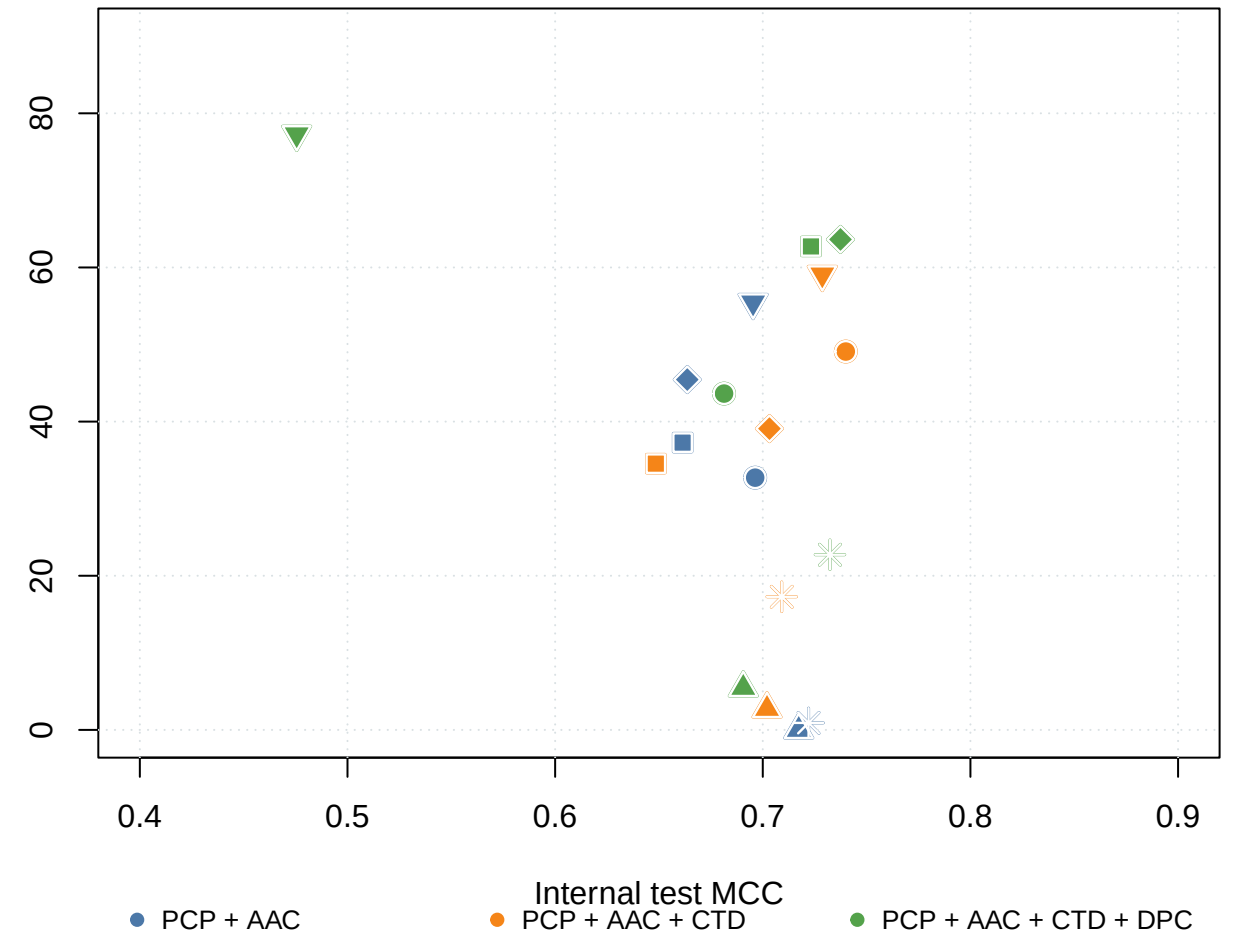
Proxy-integrated training
