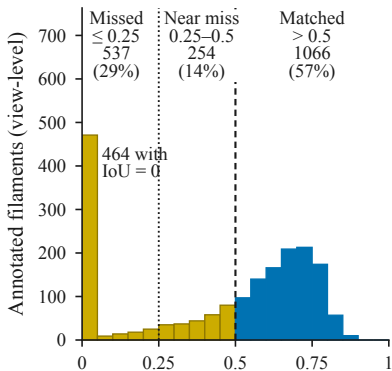
(a) Best IoU of an annotated filament with any prediction
