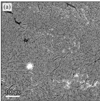
H \alpha , limb darkening removed
