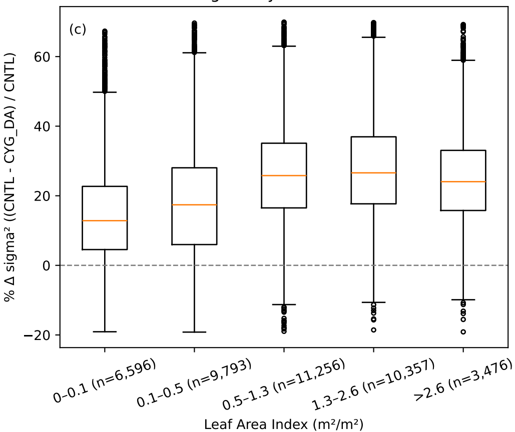
% \Delta \sigma^2 by Leaf Area Index
