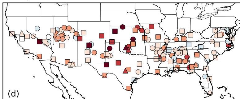
ALL_DA - CNTL
