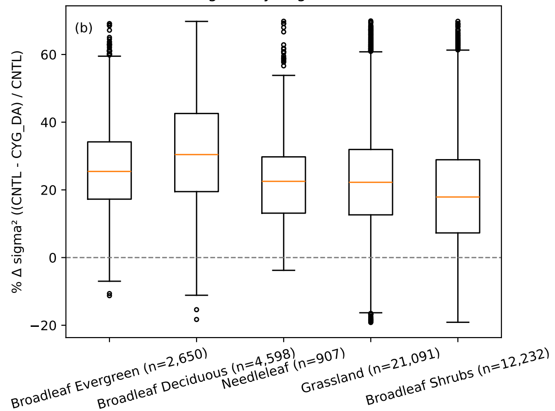
% \Delta \sigma^2 by Vegetation Class
