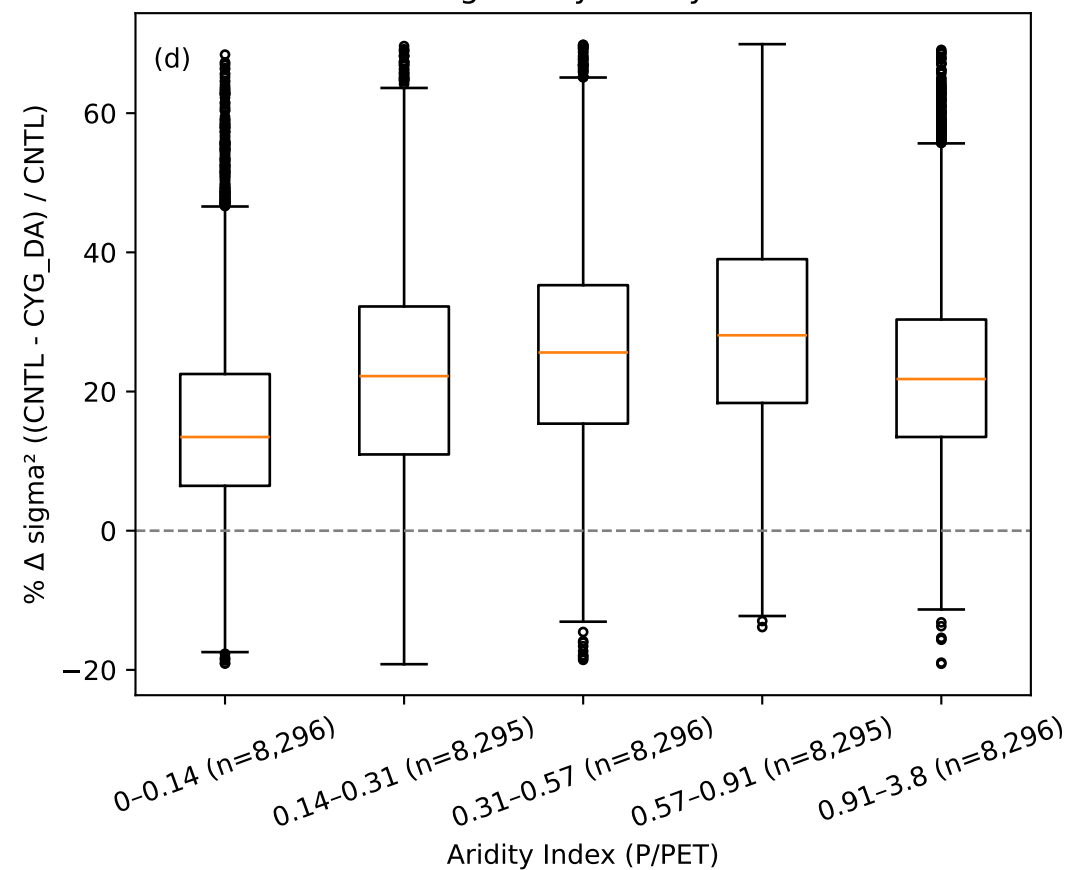
% \Delta \sigma^2 by Aridity Index
