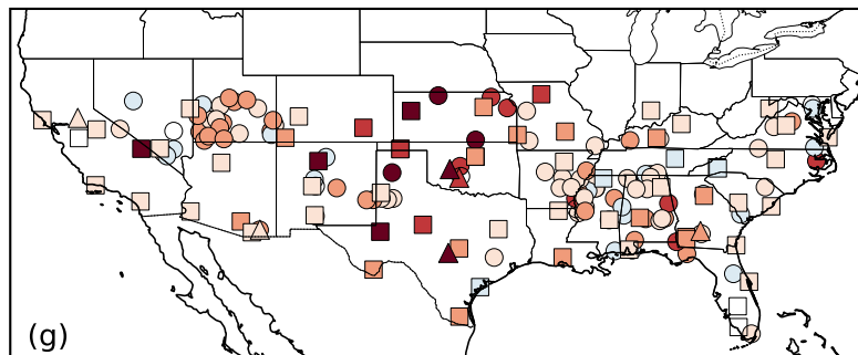
ALL_DA - CNTL
