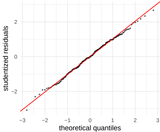
simulated normal errors (reference)
