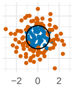
Nonlinear boundary
