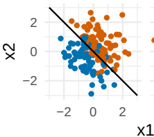
Linear boundary
