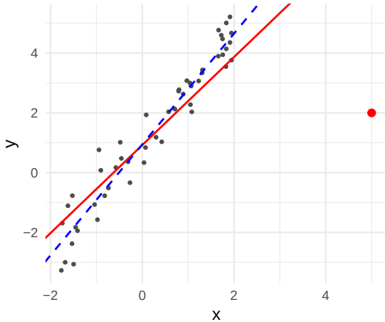
fit with (red) and without (blue) the point
