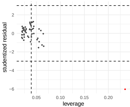
leverage vs studentized residual
