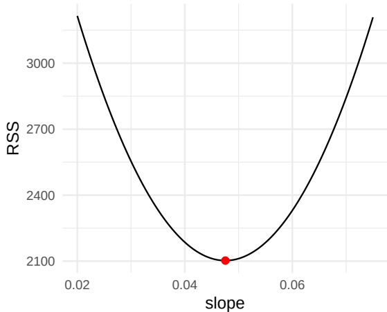
RSS as a function of the slope
