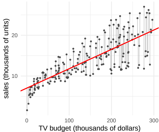
residuals: vertical distances to the line
